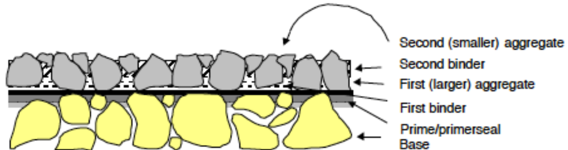
Figure 3 Components of a DBST (Source aapa Work tips 22)
