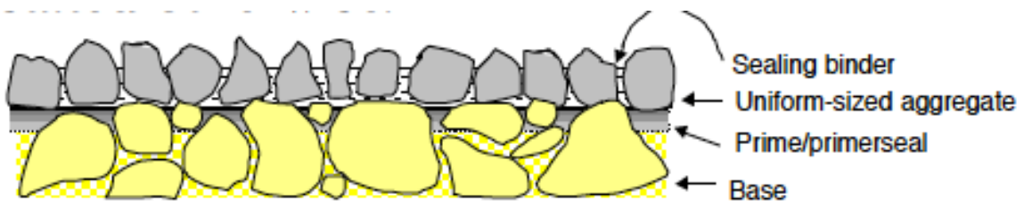
Figure 2 Components of a SBST (Source aapa Work tips 22)
